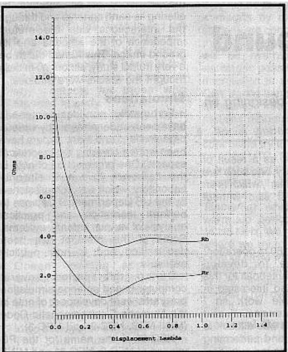
Fig 1 — 0.10 wave radiator/radials \cdot 3 @ 1.825 MHz (13,5).
